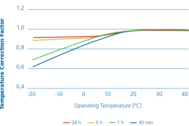
Temperature Correction Factor vs Discharge rates
