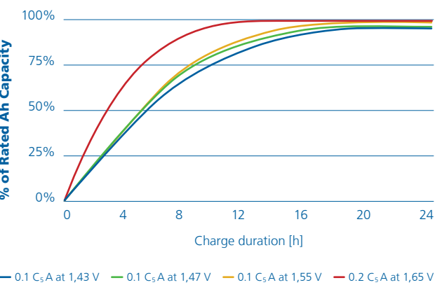
Rechargeability of GAZ® Lomain KGL cells at +20 °C
