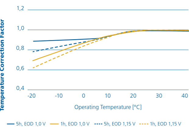
Temperature Correction Factor vs EOD Voltage
